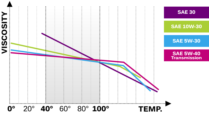
Viscosity performance
