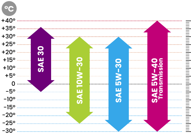
Temperature performance
